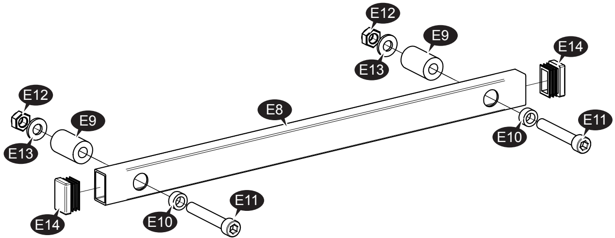
15010236 Handle Assy
