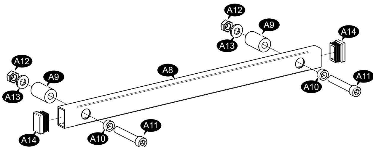
15010236 Handle Assy
