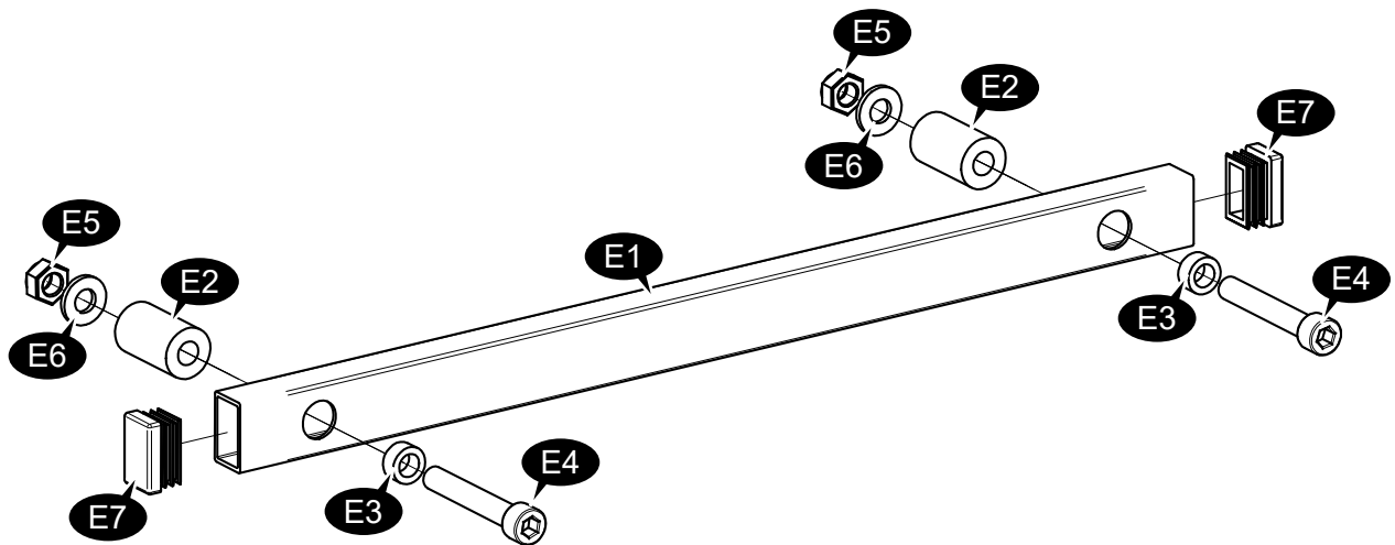
15010236 Handle Assy
