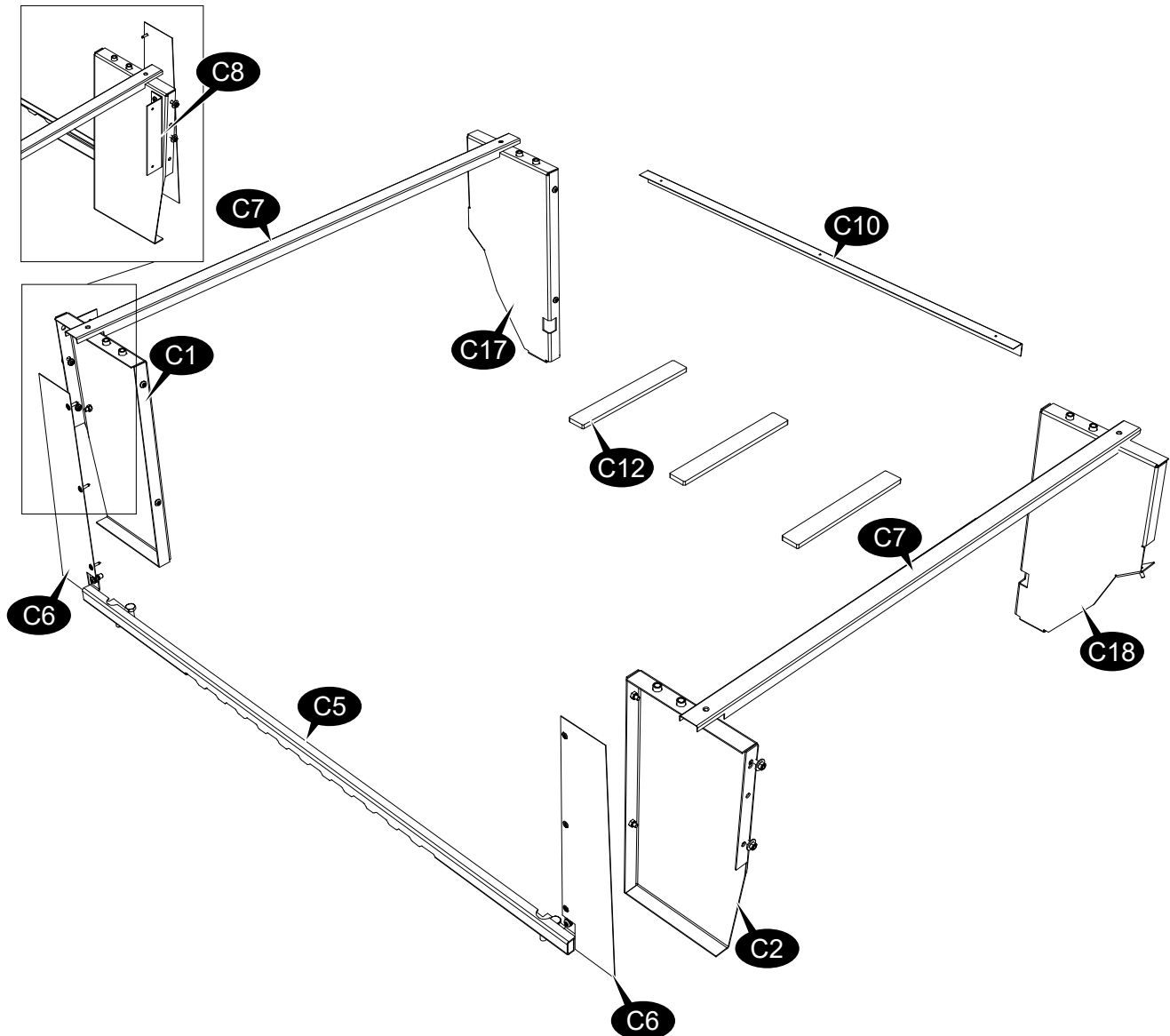
15012883 Steelbracket Set Rear Mod Drawer T6 Long
