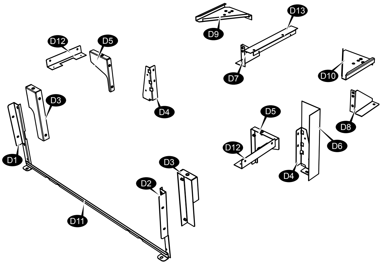
15013181 Steel Bracket Set L0 PEJ 2016
