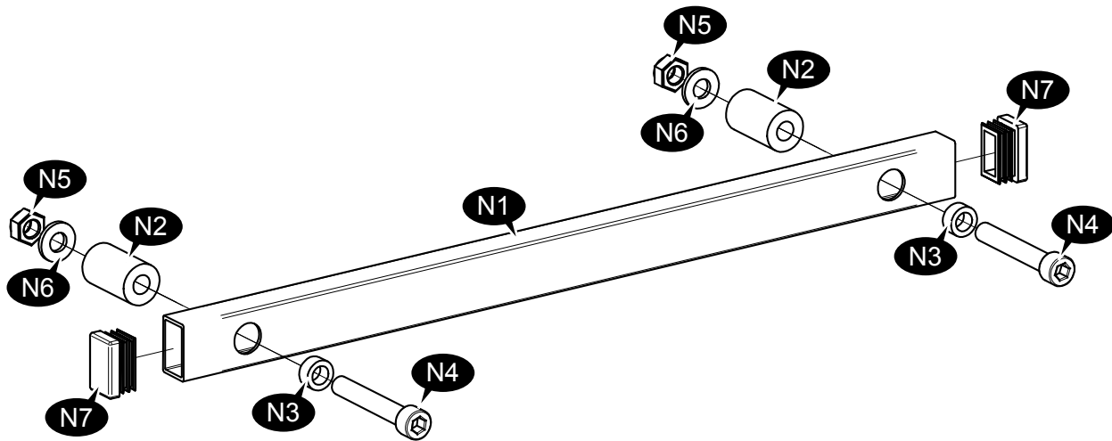
15010236 Handle Assy
