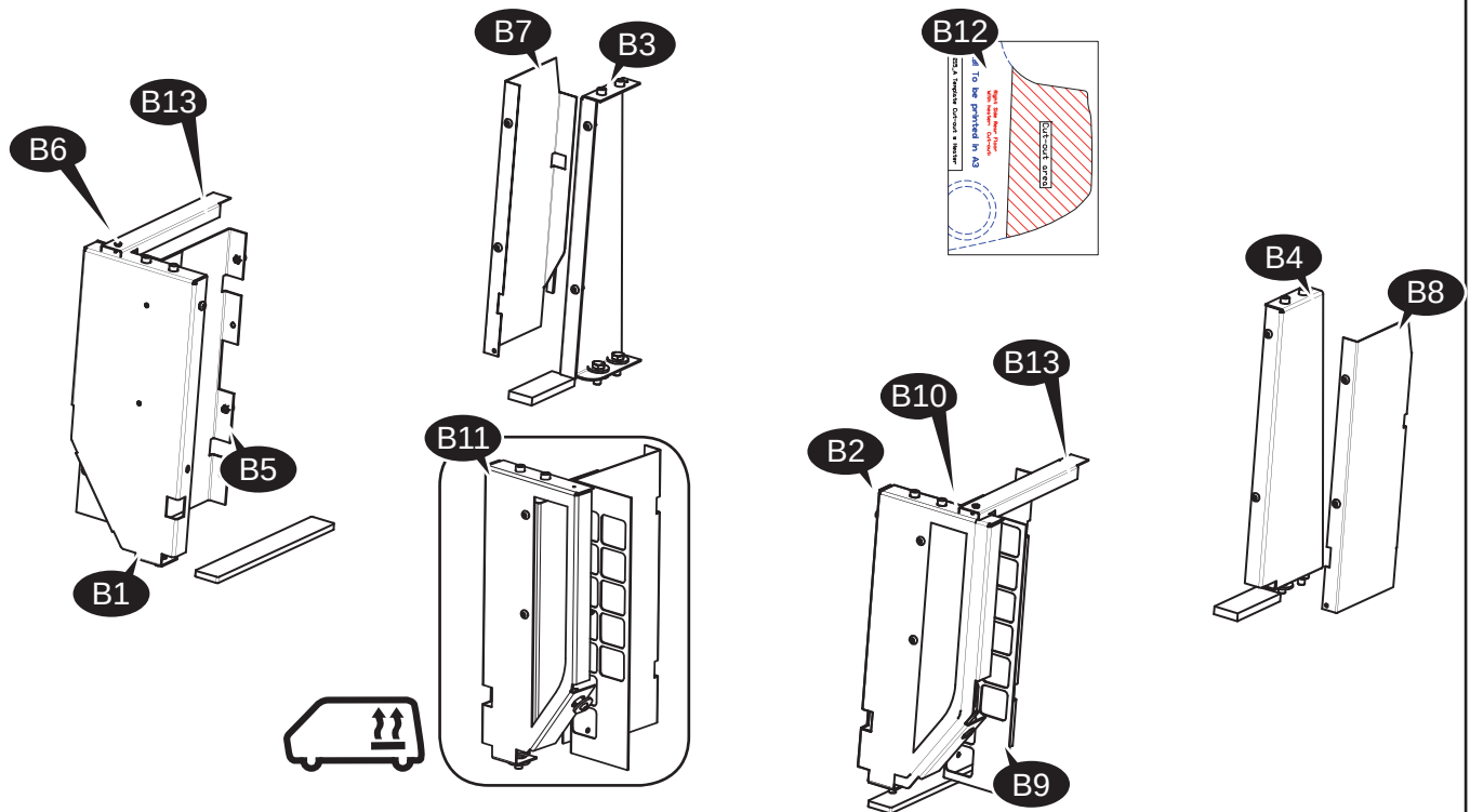
15012291_C Steelbracket Set Front Module Drawer T6
