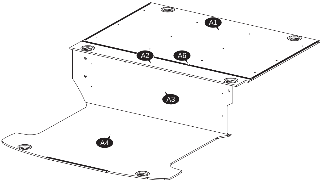
15012293_C Floor Kit Front Module drawer T6 Short
