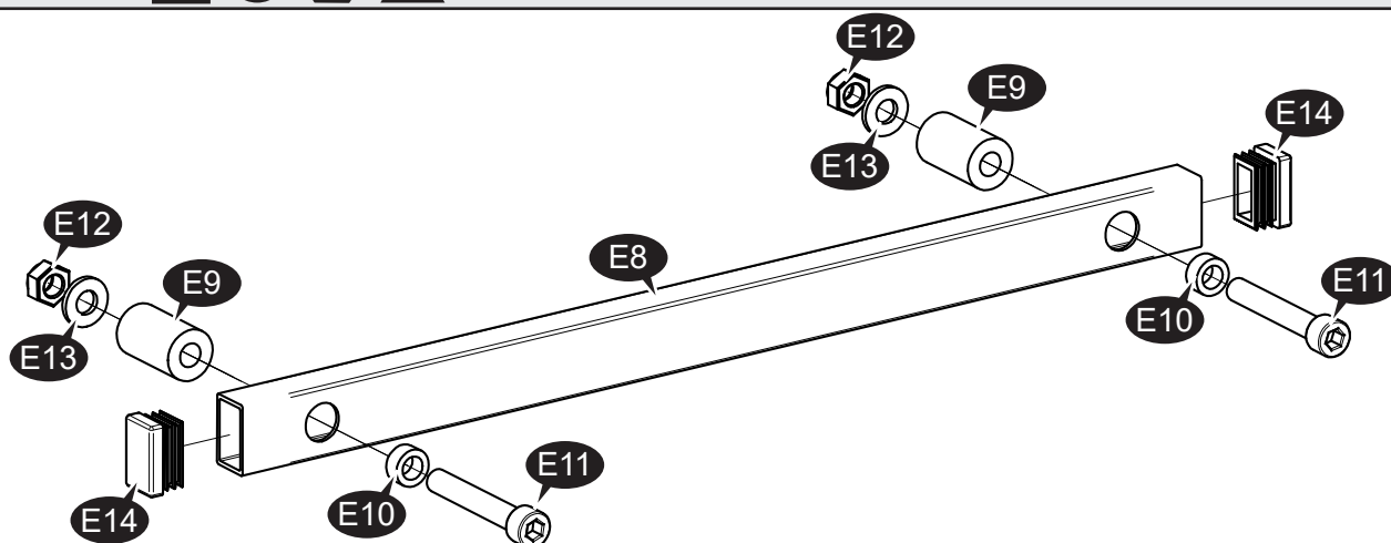
15010236 Handle Assy
